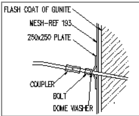
Detail 1. At the cut face.
