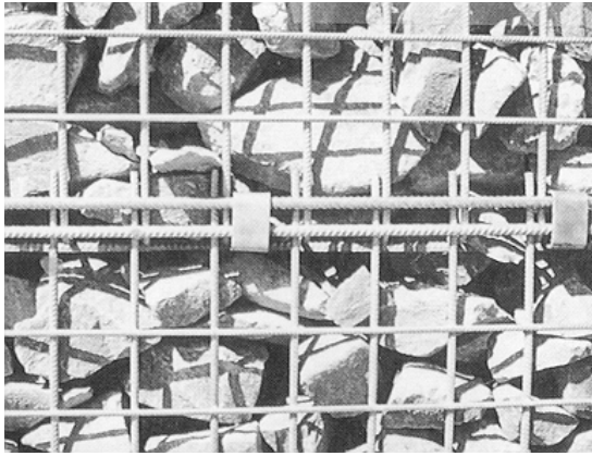
Figure 3. The TerraTrel ® cladding.
