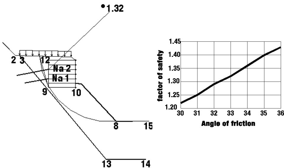
Figure 5. Overall stability analysis for 4.4 m high MSE structure.
