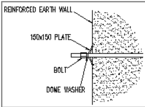
Detail 2. At the MSE cladding.
